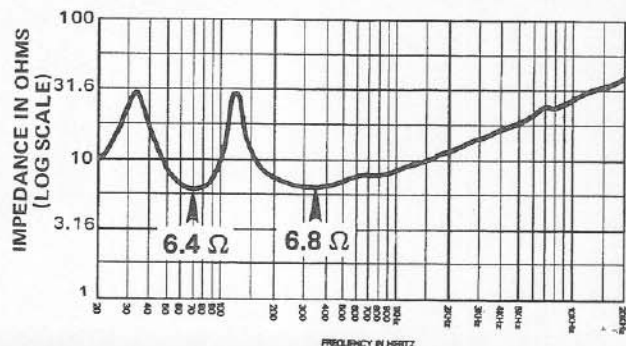
FIGURE 8 TL806/EVM.12L Input Impedance vs. Frequency
