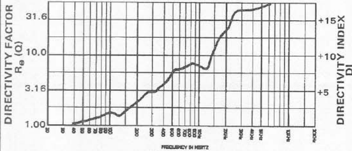
FIGURE 5 TL806/EVM.12L Directivity Factor and Directivity Index vs. Frequency
