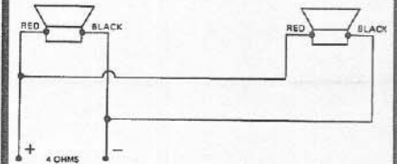
FIGURE 11 Connection of 2 EVM-12L Speakers in Parallel
