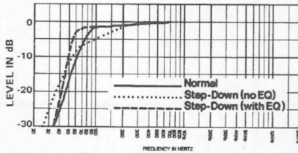
FIGURE 6 TL806/EVM.12L Low Frequency Response
