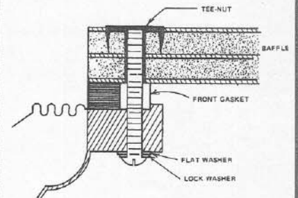
FIGURE 10 Rear Mounting Detail (Not to scale)
