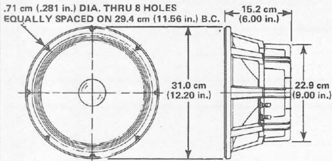
FIGURE 1 – Dimensions
