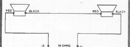
FIGURE 12 Connection of 2 EVM-12L Speakers in Series
