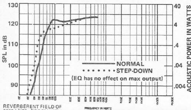
FIGURE 7 TL806/EVM.12L Theoretical Low Frequency Maximum Acoustic Output vs. Frequency
