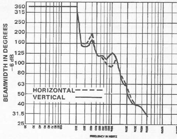
FIGURE 4 TL806/EVM.12L Beamwidth vs. Frequency
